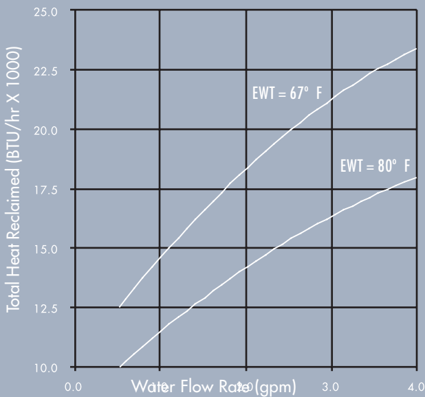
Enviro-Pak Heat Recovery Rate
